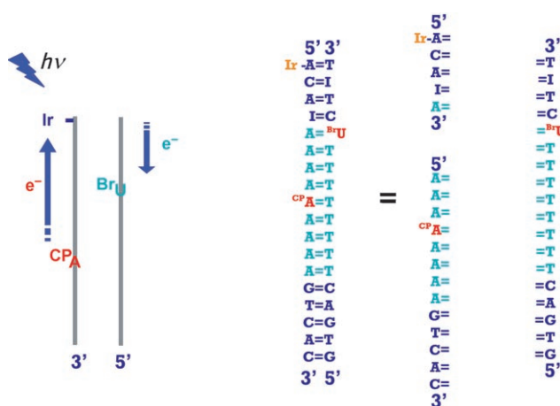
Scheme 2. The assembly of three modified DNA single strands annealed to generate the Ir–DNA duplex for the ping-pong reaction.
